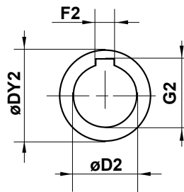
Hollow shaft
