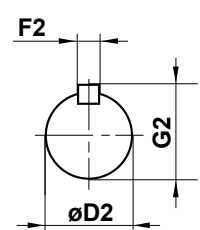
Output shaft
